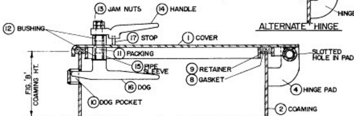
SECTION
