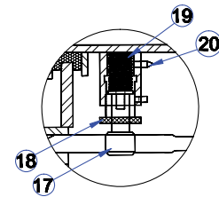
DETAIL OF SWIVEL GUIDE AREA
