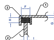
SECTION A-A Gasket Groove Detail
